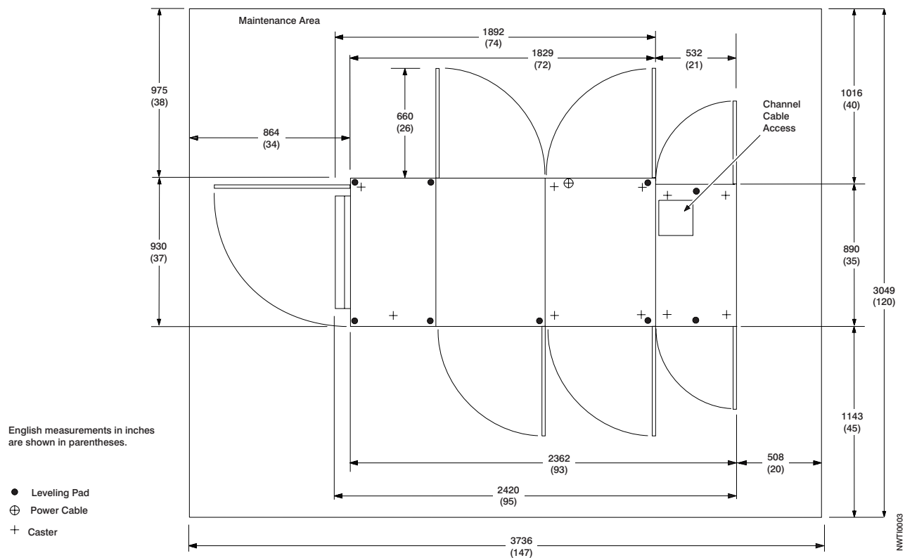
Figure 5-2. Dimensions, Service Clearance, Power cable, and Cable Locations—Models IS1 and IS2
