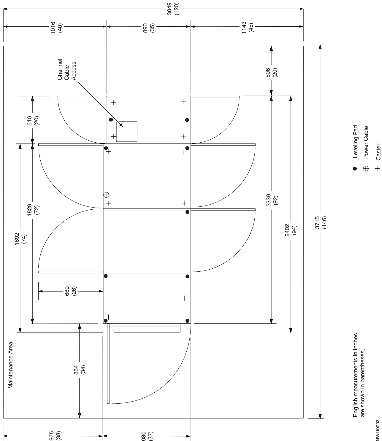
Figure 5-3. Dimensions, Service Clearance, Power cable, and Cable Locations—Models 0W1 and 0W3
