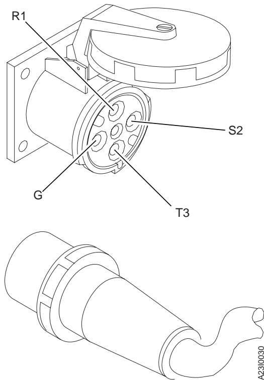
Figure 5-1. Hubbell Plug and Receptacle. Positions for phase connectors R1, S2, T3, and ground (G) are shown.
