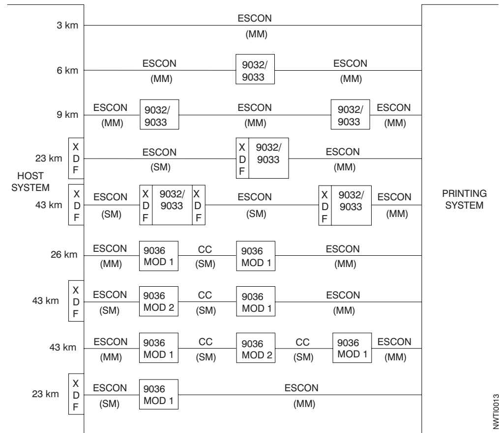
Figure 4-2. Serial Channel Attachment Options
