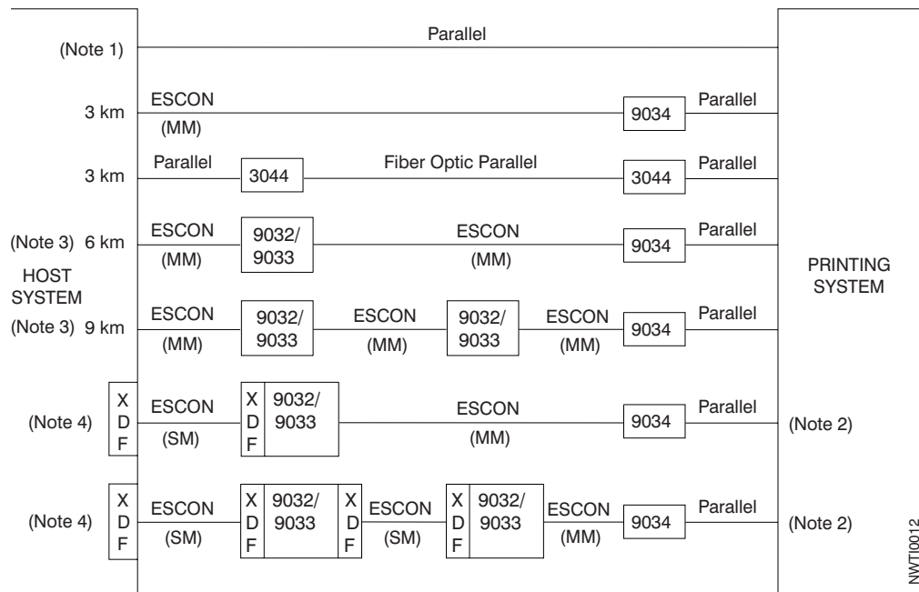
Figure 4-1. System/370 Parallel Channel Attachment Options
