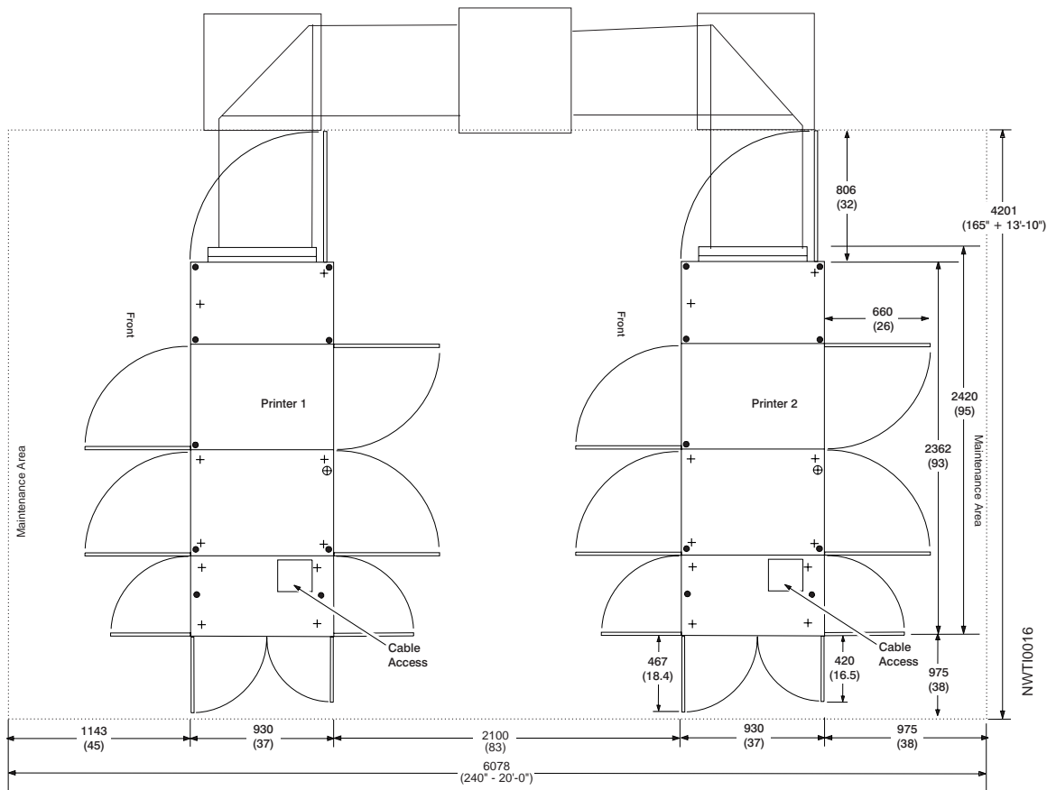
Figure 5-10. 'h' Configuration (Both Printers Facing the Same Direction)
