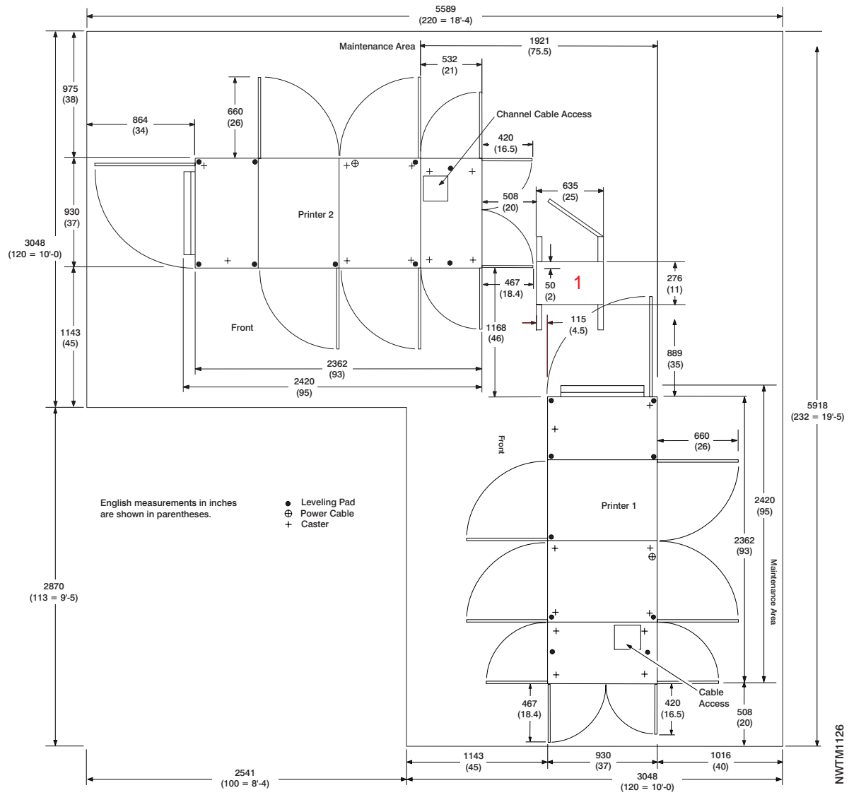
Figure 5-9. ID3/ID4 Left Angle Configuration
