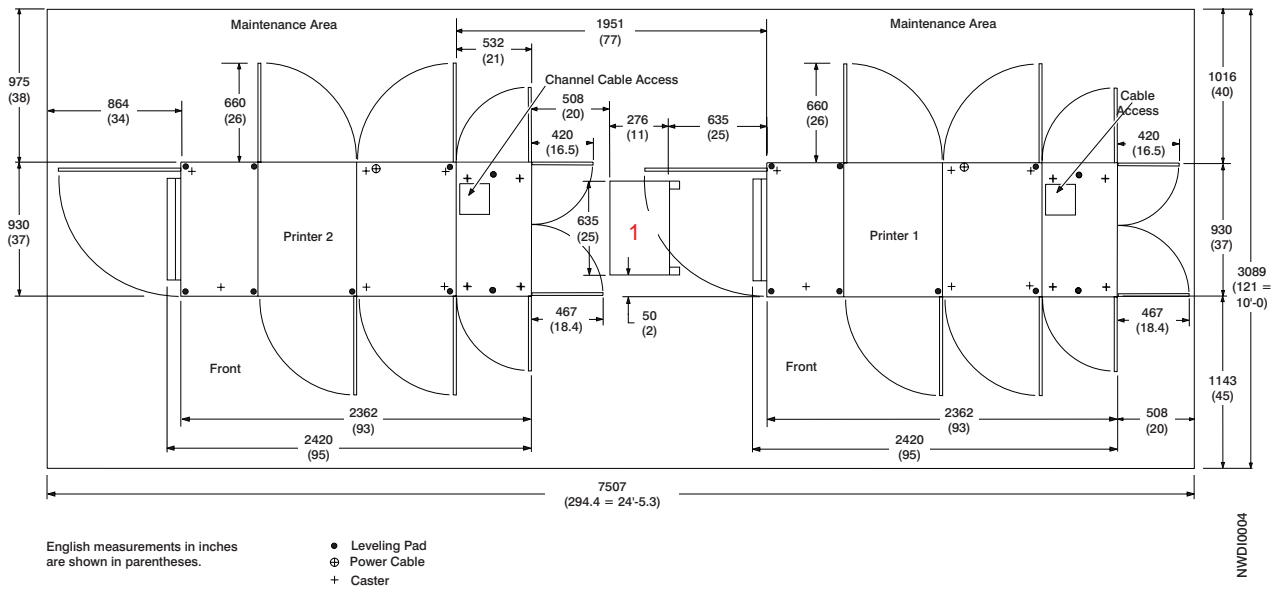
Figure 5-6. DR1/DR2, ID1/ID2, IR1/IR2, and IR3/IR4 Inline Configuration
