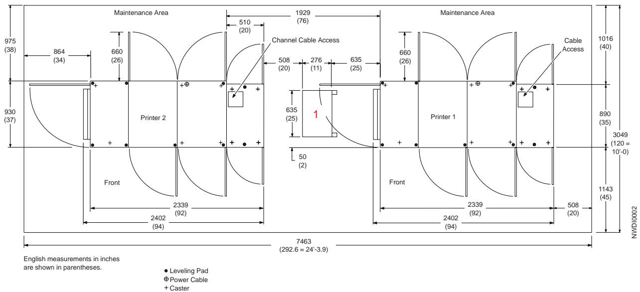
Figure 5-4. D01/D02 and DW1/DW2 Inline Configuration
