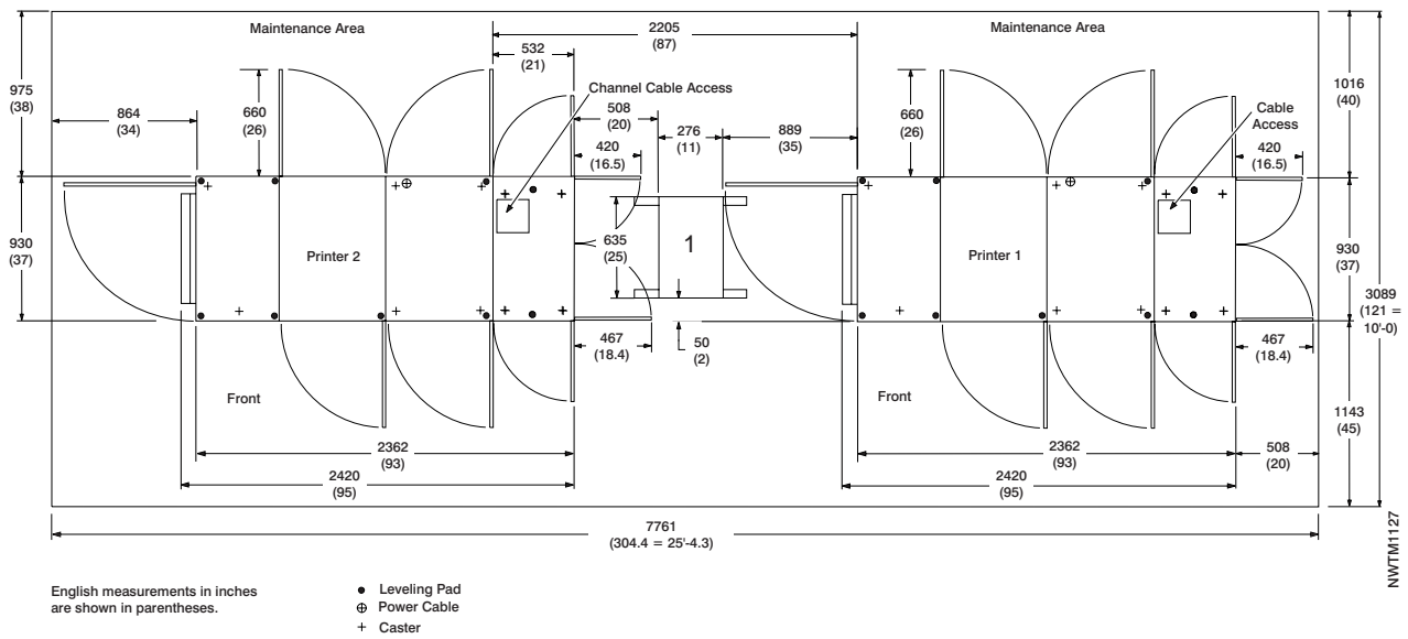
Figure 5-8. ID3/ID4 Inline Configuration
